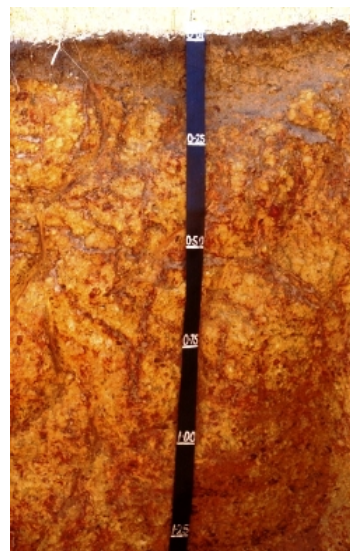
Shallow gravel (Narrogin)
