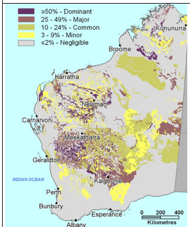
544 Red loamy earth p 134
