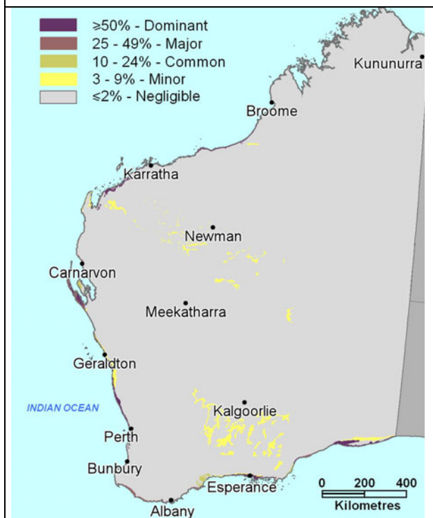
442 Calcareous deep sand p 86
