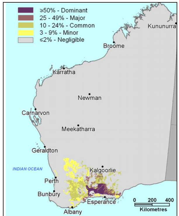
402 Alkaline grey shallow sandy duplex p 60
