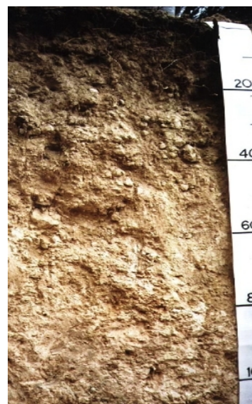
Calcareous loamy earth (Mount Beaumont)
