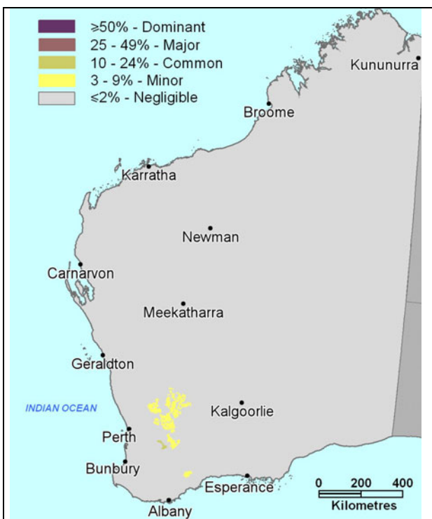
501 Acid shallow duplex p 106
