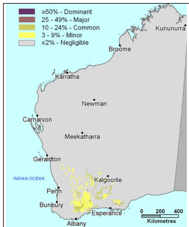
502 Alkaline grey shallow loamy duplex p 108
