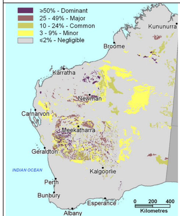
423 Red shallow sand p 80
