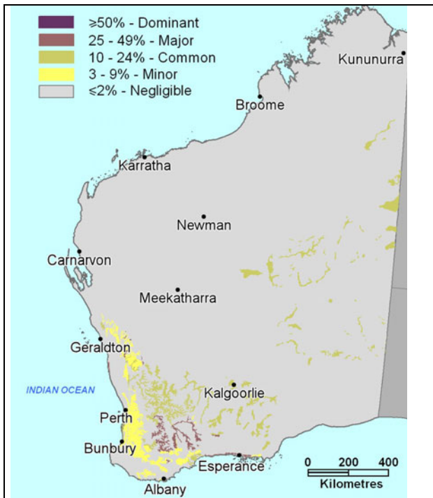
101 Saline wet soil p 34
