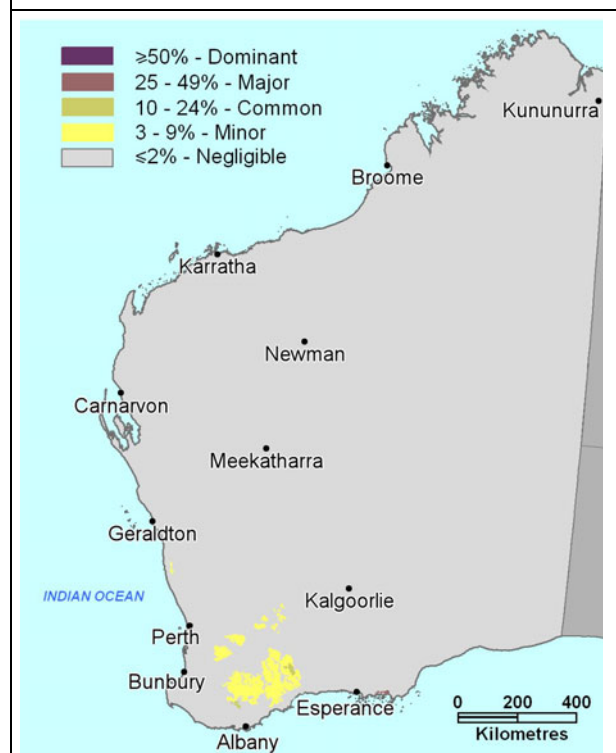
504 Grey shallow loamy duplex p 112
